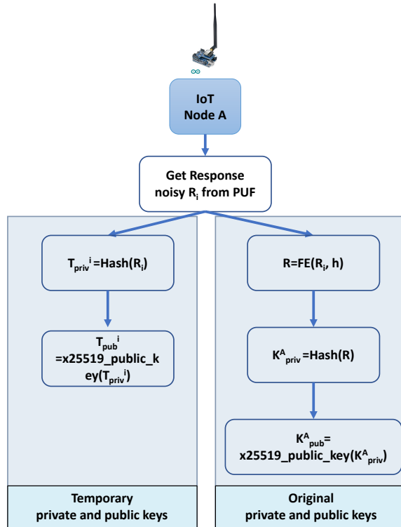
Figure 1: Generation of original private and public keys from reconstructed response and temporary keys from unstable responses.
